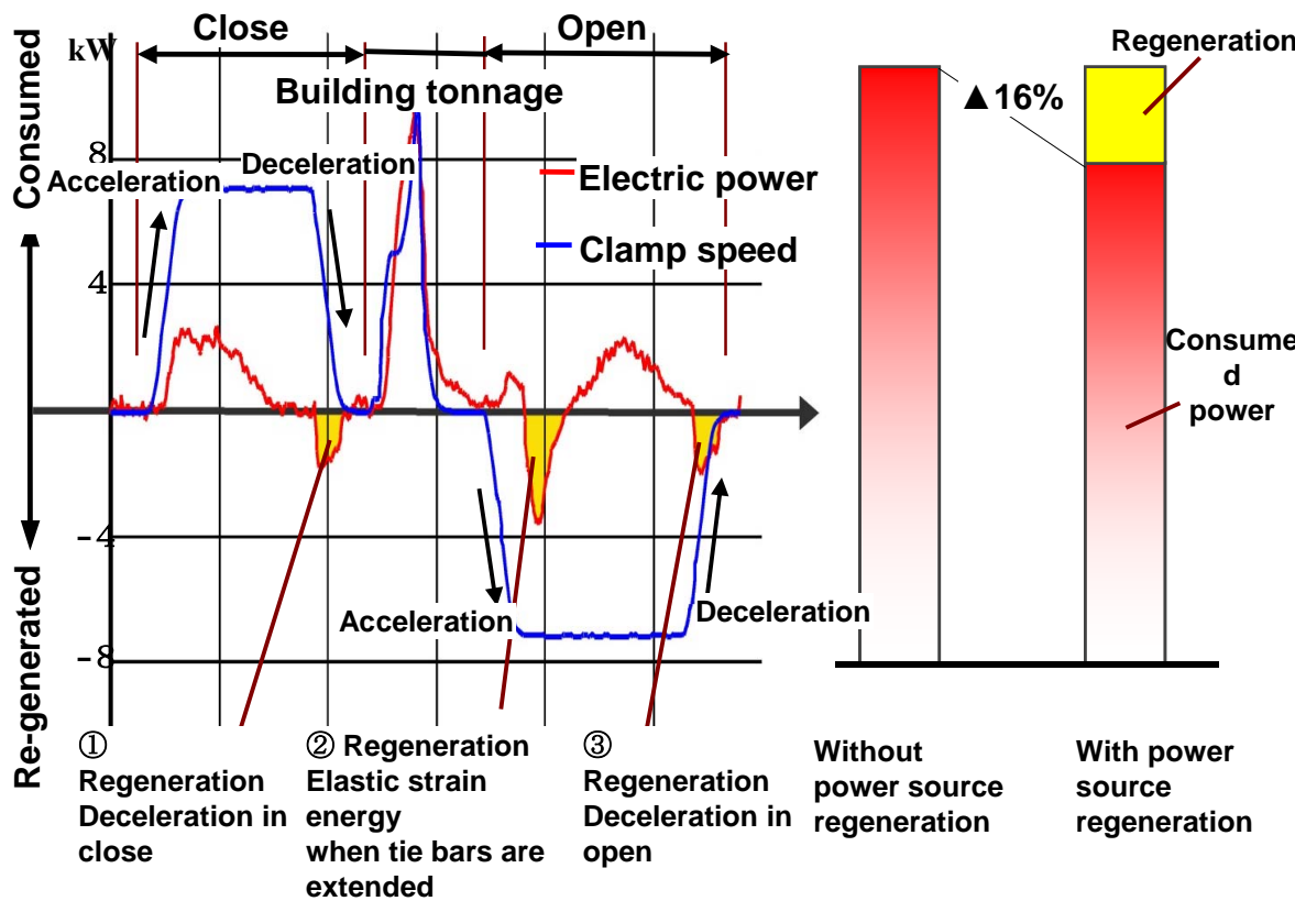
Power consumed during clamp open/close (100-t)
